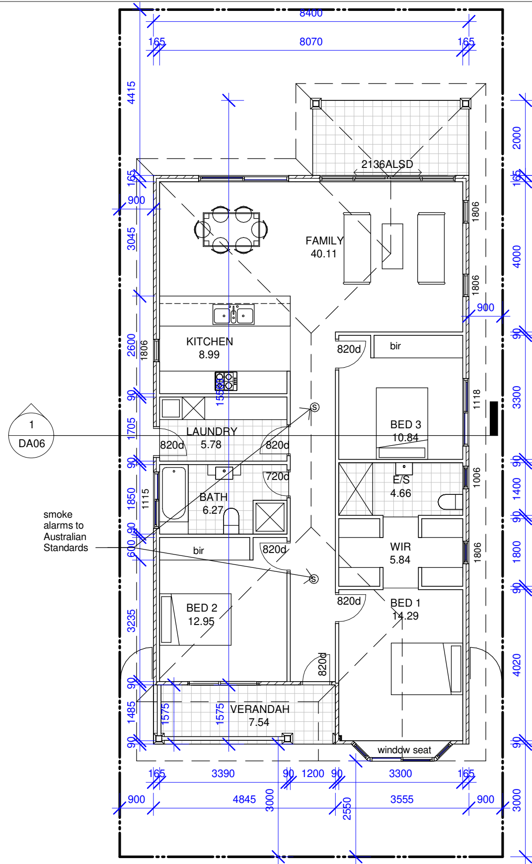
1 GROUND FLOOR PLAN 1 : 100
