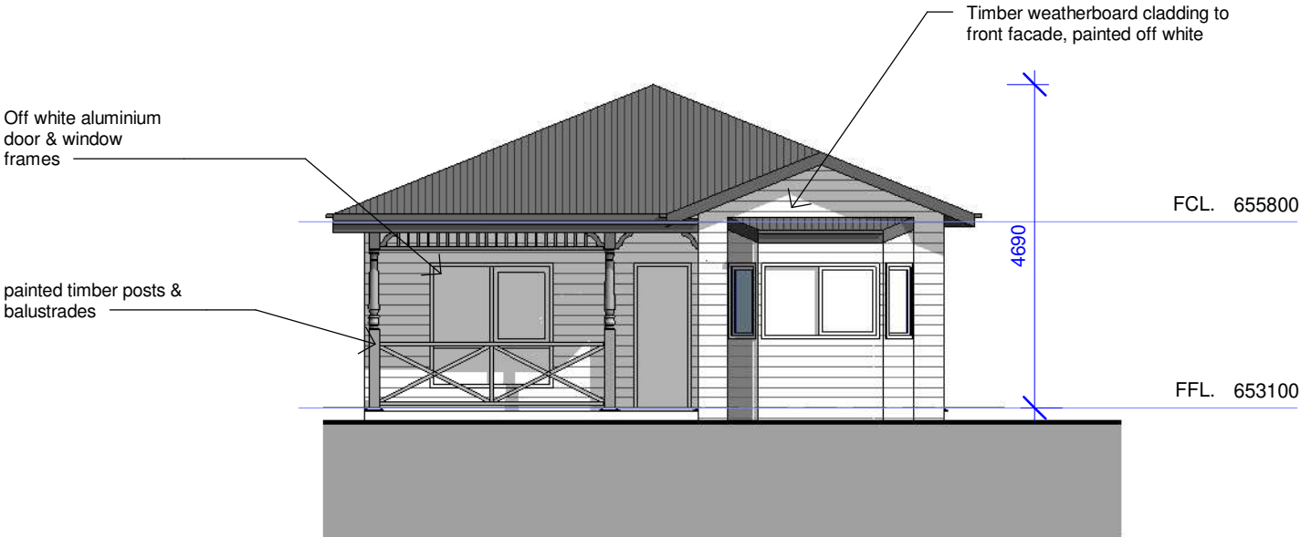
1 SOUTH ELEVATION 1 : 100
