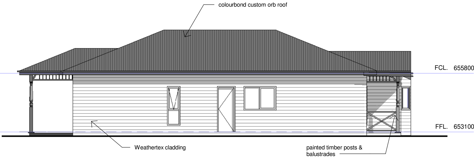
2 WEST ELEVATION 1 : 100
