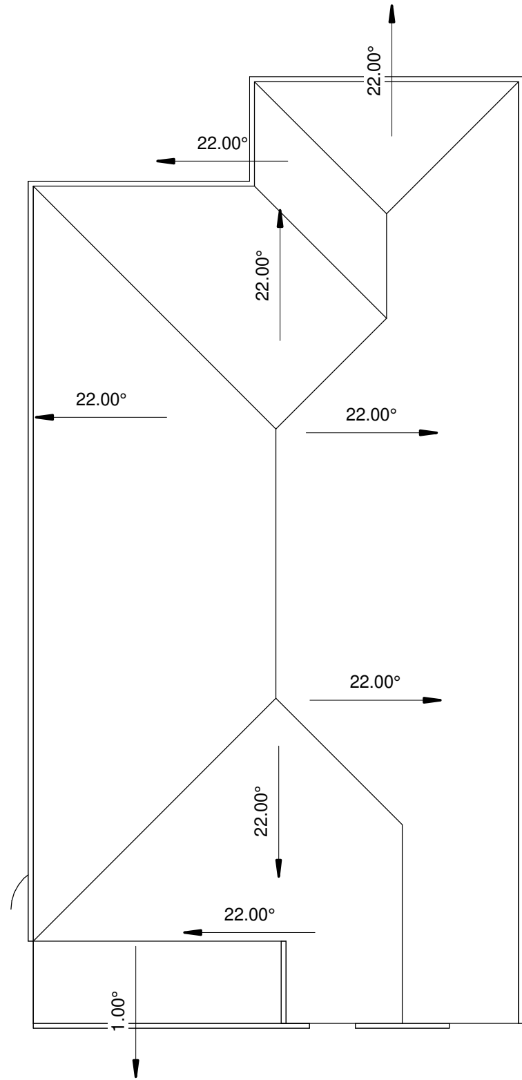
1 ROOF PLANS 1 : 100
